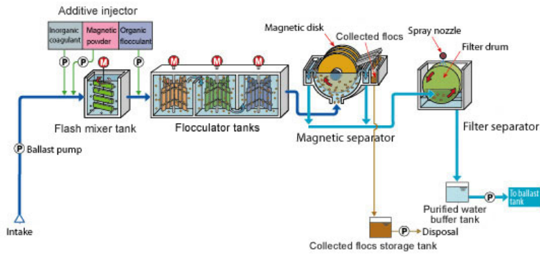
System flow
