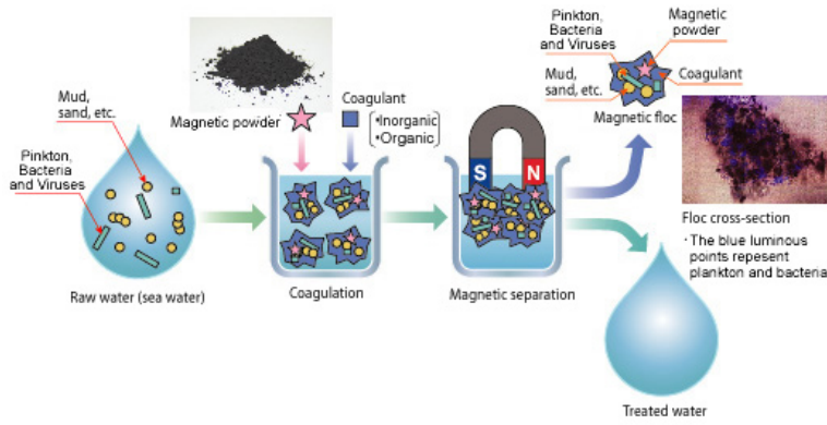
Process outline
