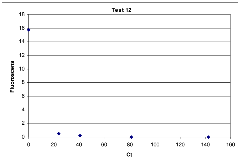
Figure 4. In vivo fluorescens measurements of Pymnesium cultures treated with ozone.
