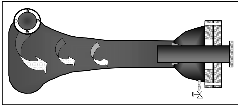
Figure 1: MicroKill separator.
