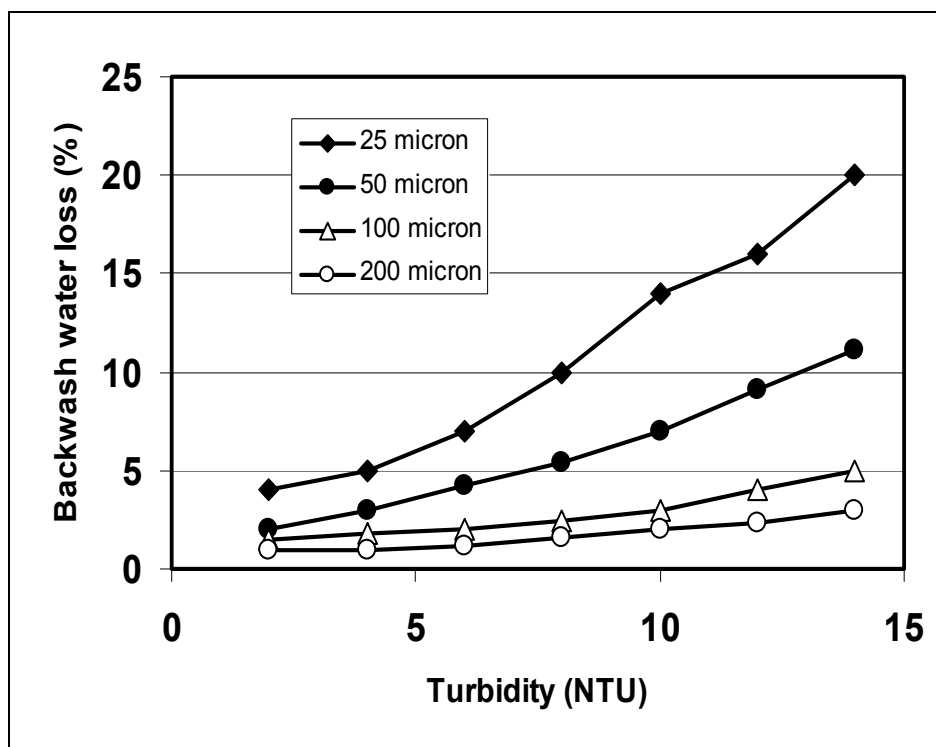
Figure 5. Backwash water loss under different solids loading conditions (flux: 60 \text{ M}^3/\text{M}^2/\text{Hr} ; line pressure: 3 bar).
