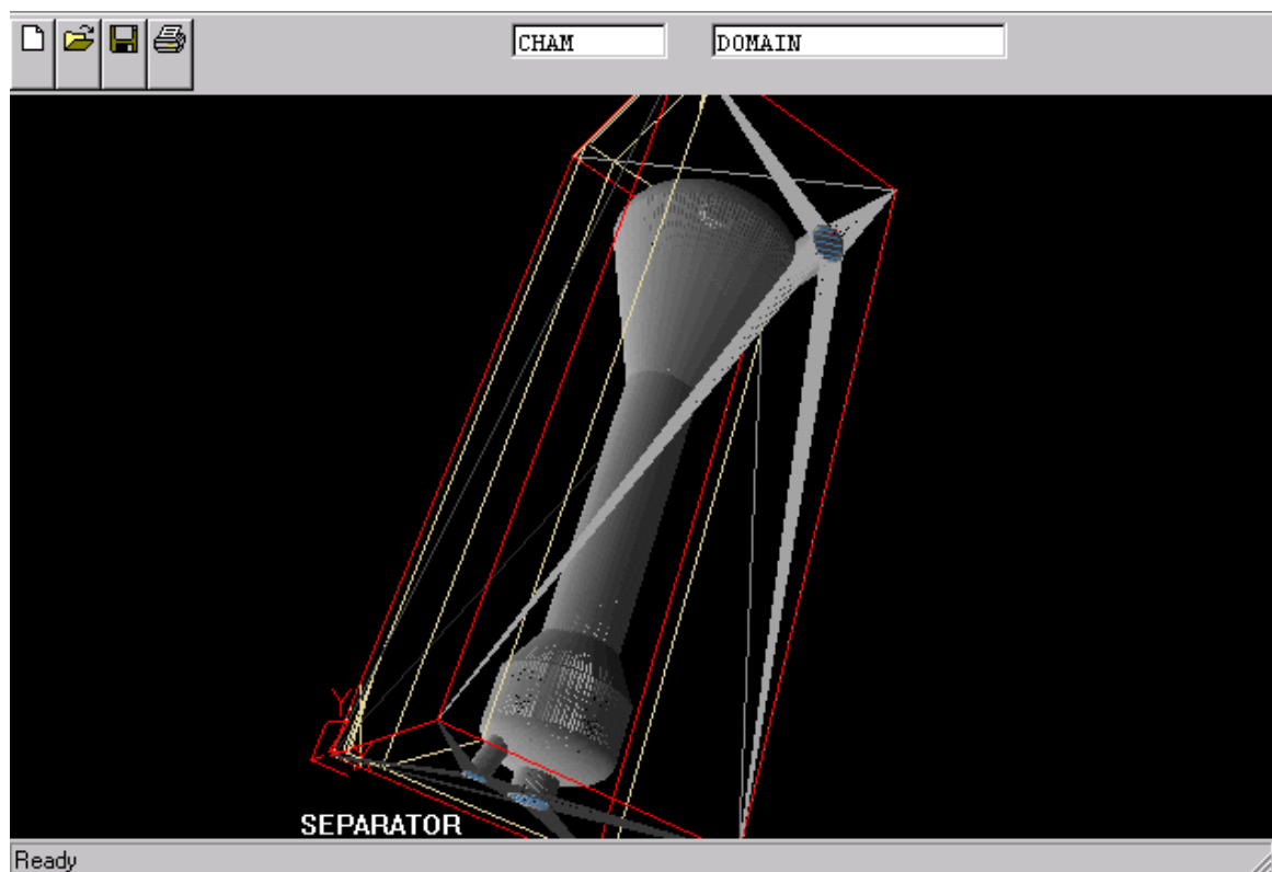
Figure 2: The Separator as a CFD model
